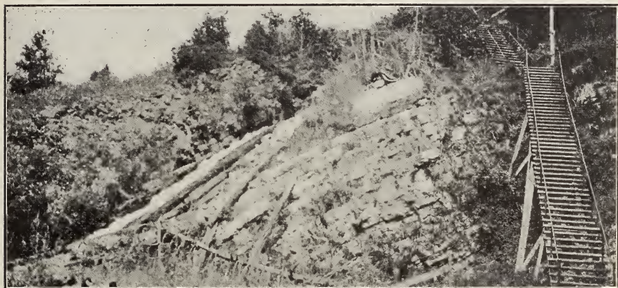
FIG. 53 ILLUSTRATING UNCONFORMABLE STRATA. CONTORTED SCHIST. ST. LAWRENCE, NEAR BEAUPRE, P. Q. (Photo by Allen.)
